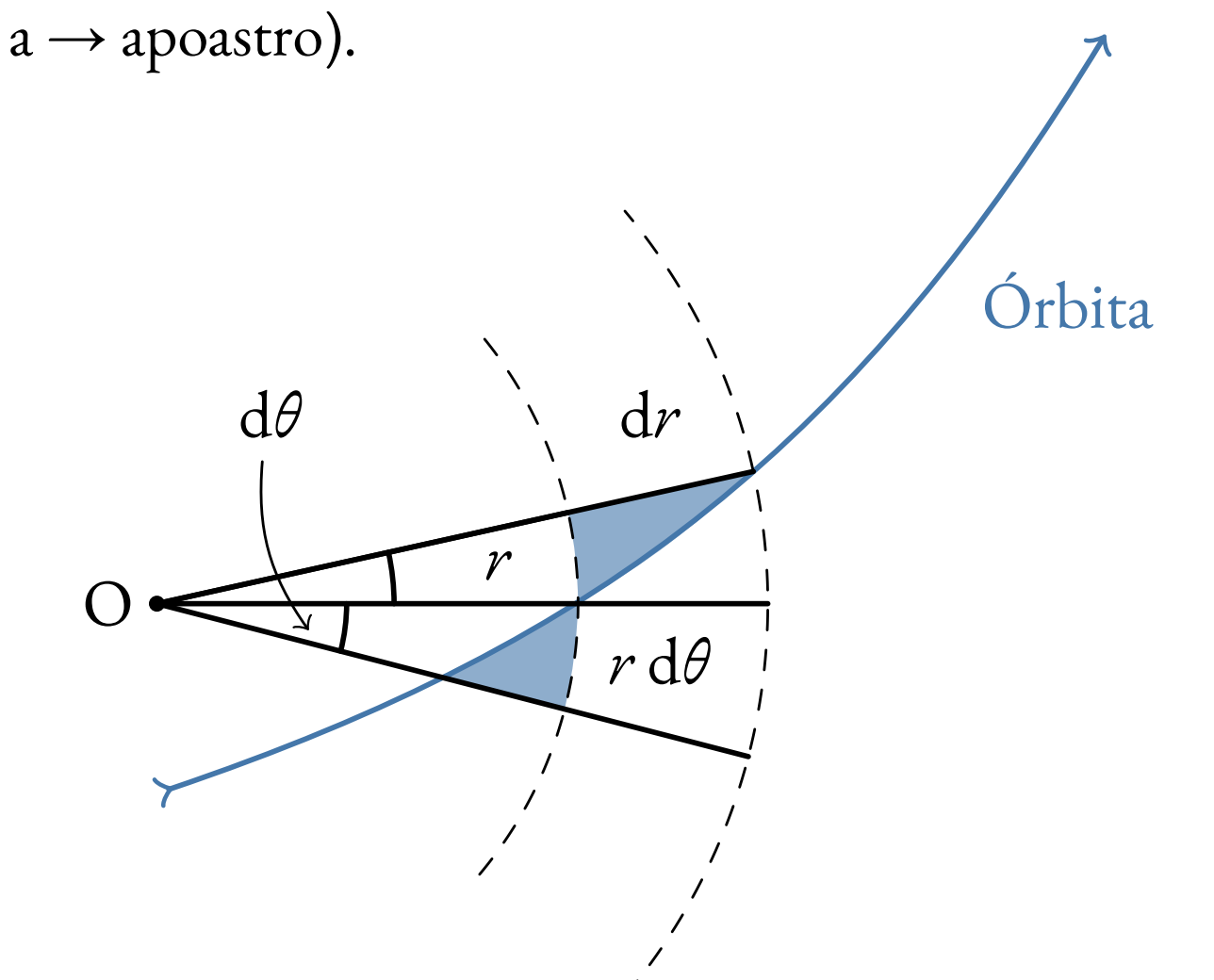
Adaptada de https://tikz.net/kepler-second-law/ .
